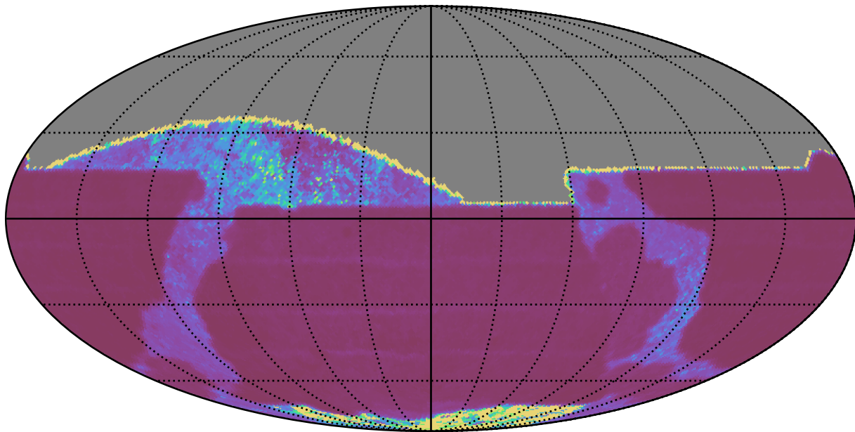
weather_cloudso35v3.4_10yrs All sky z band: Median Inter-Night Gap
