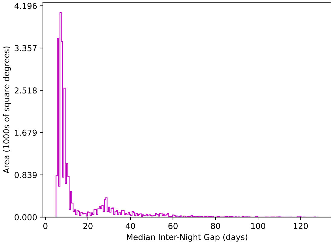
weather_cloudso35v3.4_10yrs All sky z band: Median Inter-Night Gap
