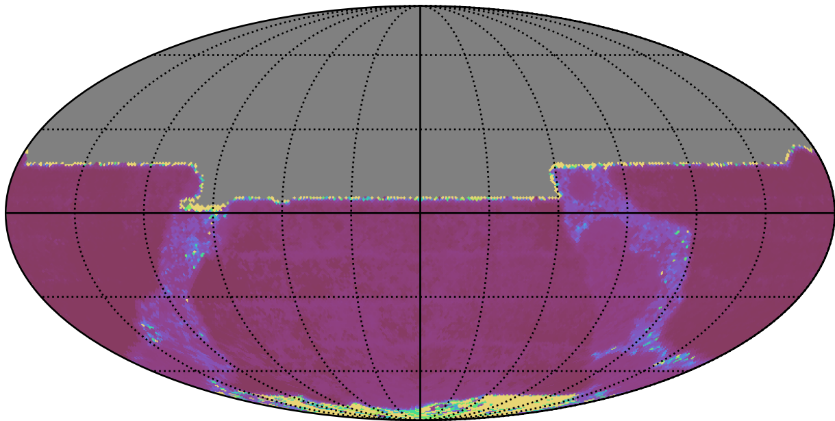
weather_cloudso35v3.4_10yrs All sky y band: Median Inter-Night Gap
