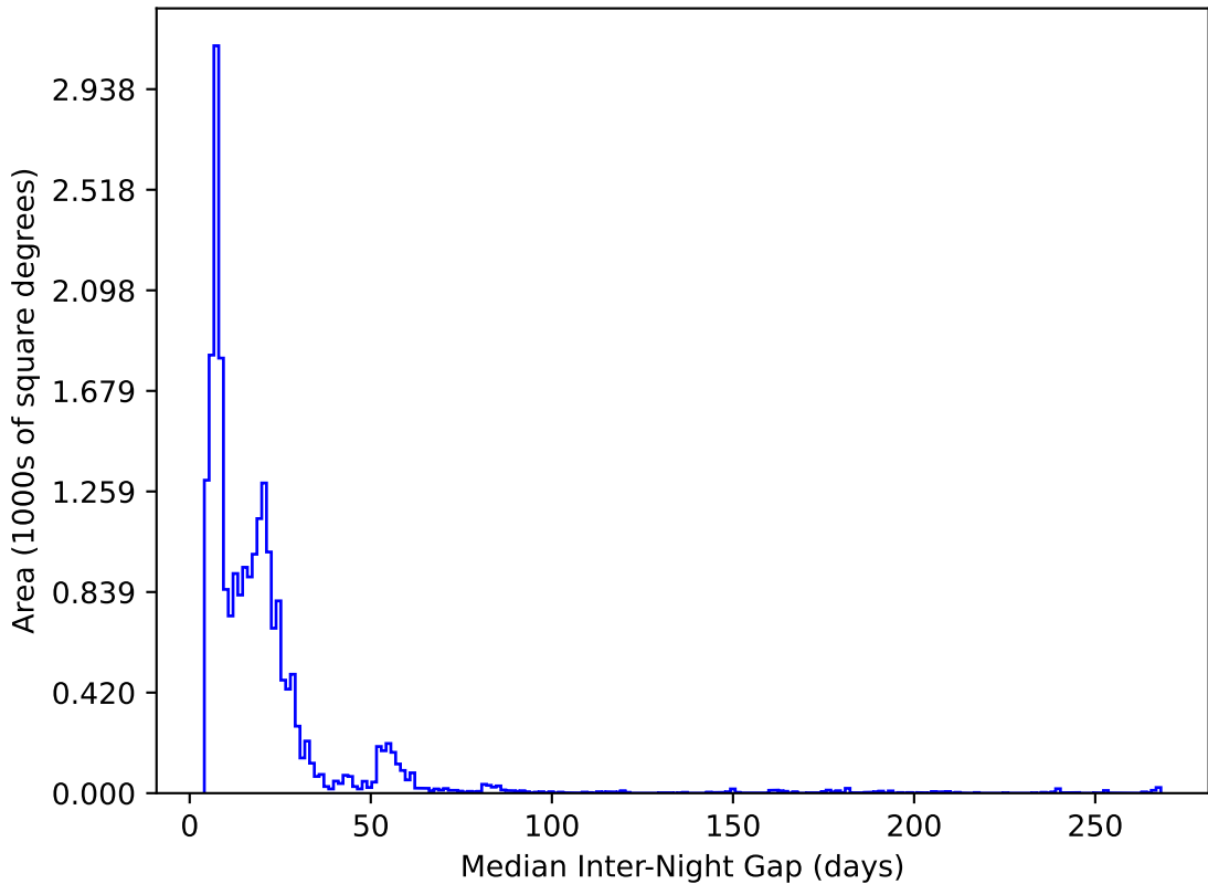
weather_cloudso35v3.4_10yrs All sky y band: Median Inter-Night Gap
