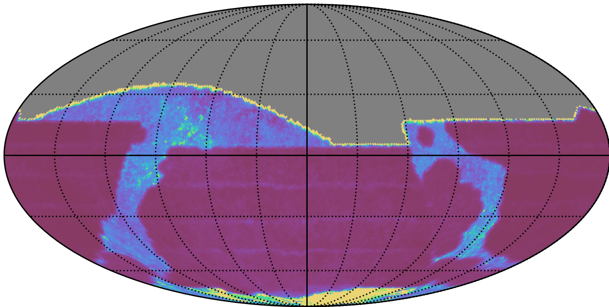
weather_cloudso35v3.4_10yrs All sky r band: Median Inter-Night Gap
