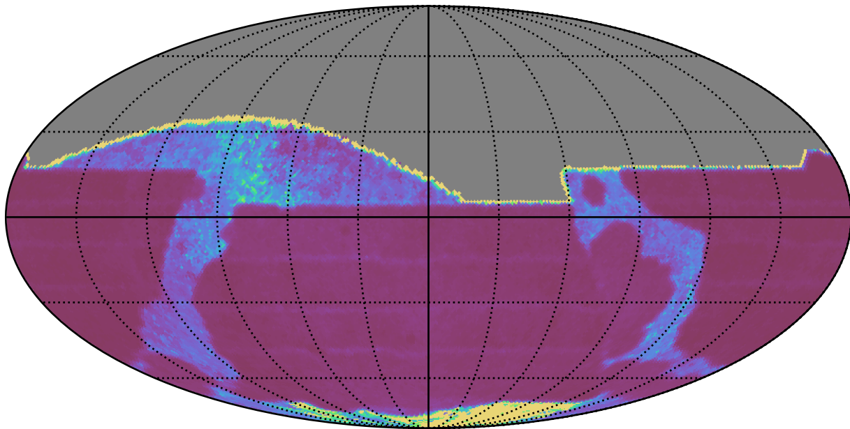
weather_cloudso35v3.4_10yrs All sky i band: Median Inter-Night Gap
