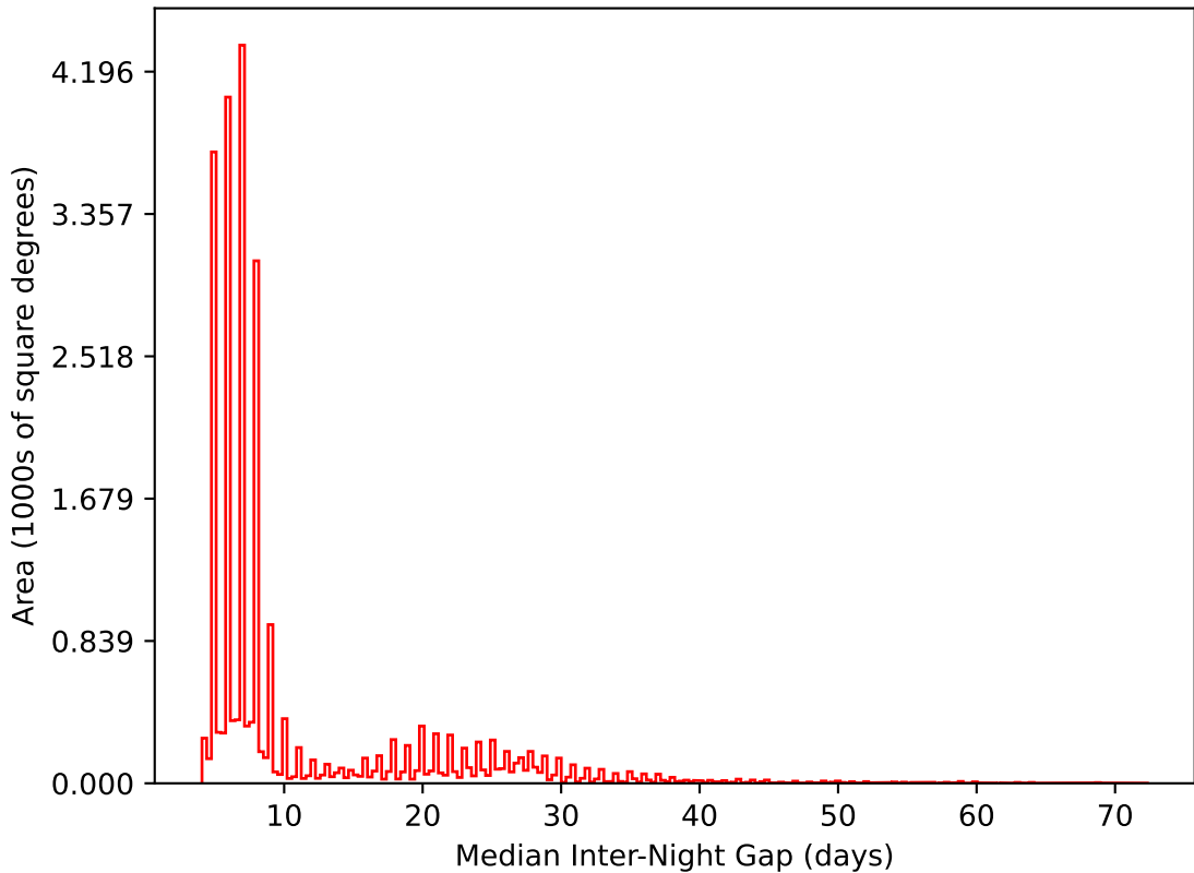
weather_cloudso35v3.4_10yrs All sky i band: Median Inter-Night Gap
