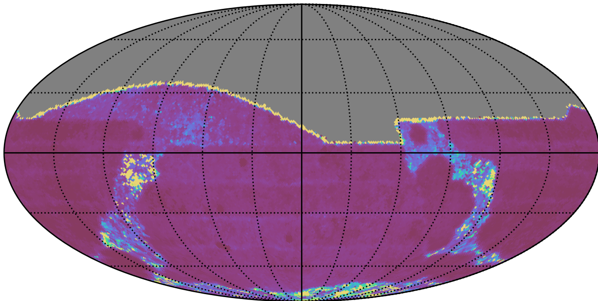
weather_cloudso35v3.4_10yrs All sky g band: Median Inter-Night Gap
