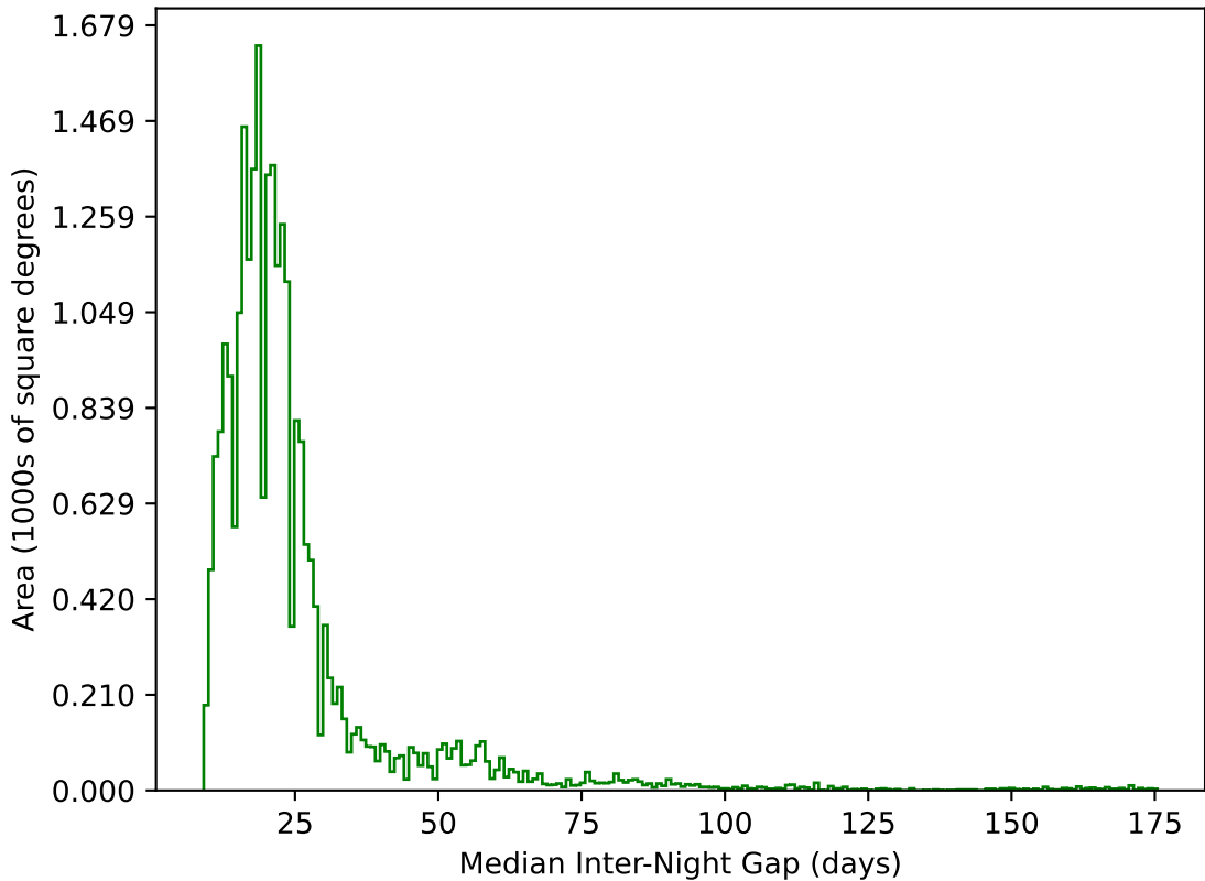
weather_cloudso35v3.4_10yrs All sky g band: Median Inter-Night Gap
