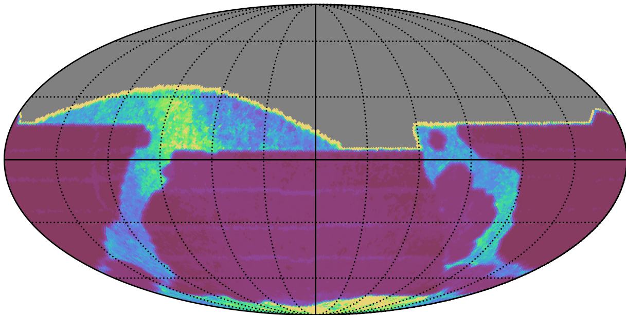
weather_cloudso35v3.4_10yrs All sky all bands: Median Inter-Night Gap
