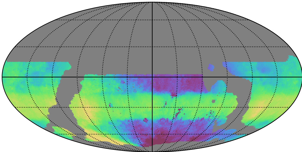
weather_cloudso35v3.4_10yrs WFD z band: Median HA
