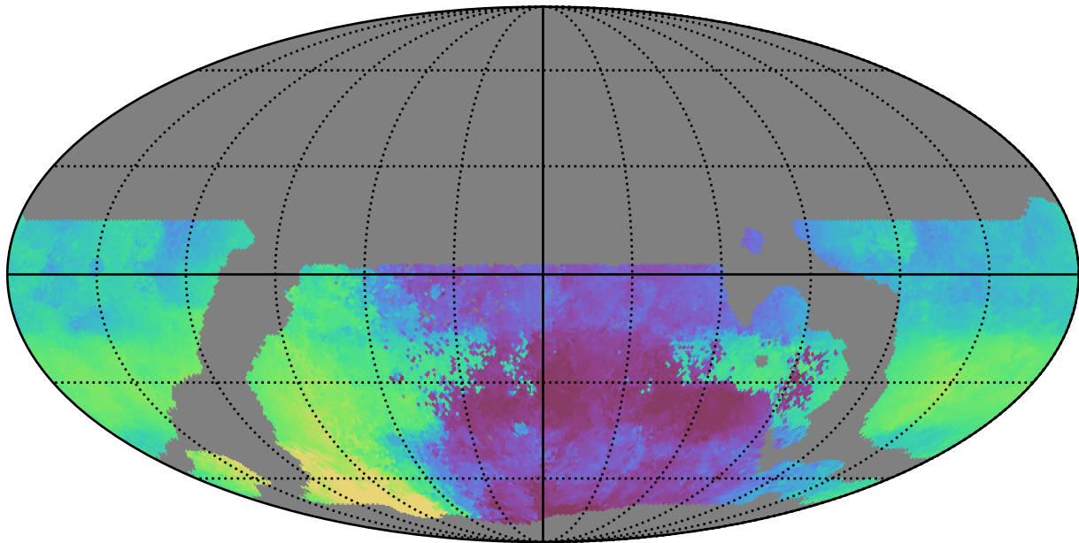
weather_cloudso35v3.4_10yrs WFD u band: Median HA
