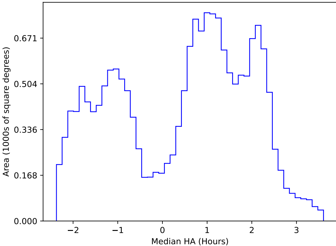
weather_cloudso35v3.4_10yrs WFD u band: Median HA
