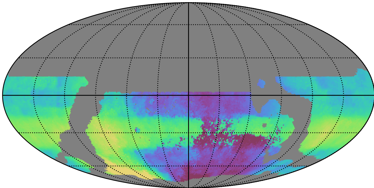
weather_cloudso35v3.4_10yrs WFD r band: Median HA
