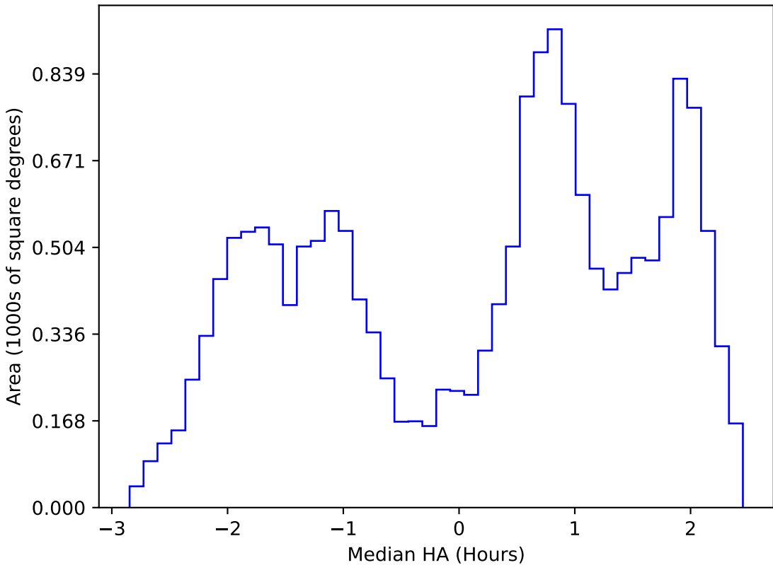
weather_cloudso35v3.4_10yrs WFD g band: Median HA
