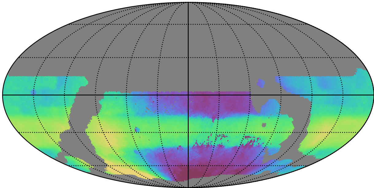
weather_cloudso35v3.4_10yrs WFD all bands: Median HA
