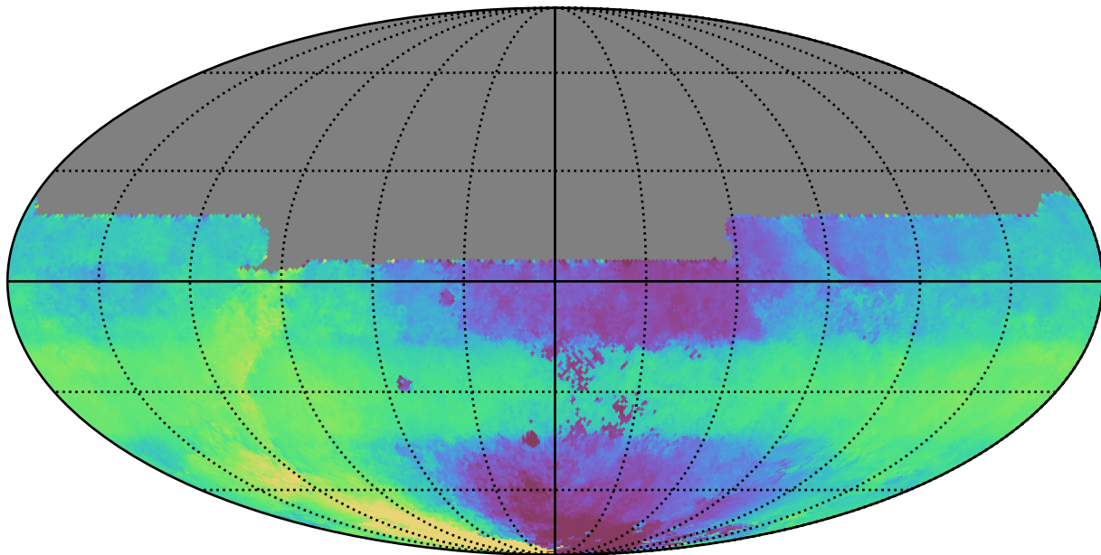
weather_cloudso35v3.4_10yrs All sky y band: Median HA
