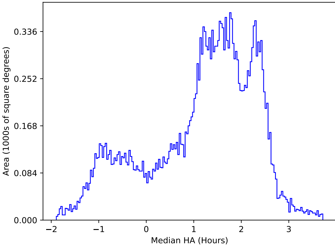
weather_cloudso35v3.4_10yrs All sky y band: Median HA
