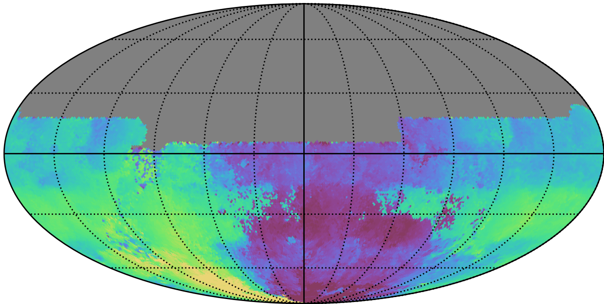
weather_cloudso35v3.4_10yrs All sky u band: Median HA
