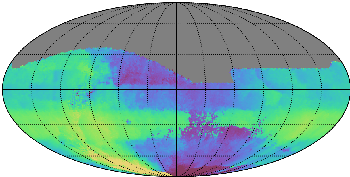
weather_cloudso35v3.4_10yrs All sky r band: Median HA
