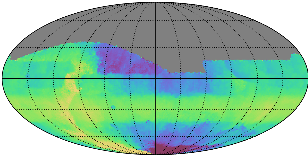
weather_cloudso35v3.4_10yrs All sky i band: Median HA
