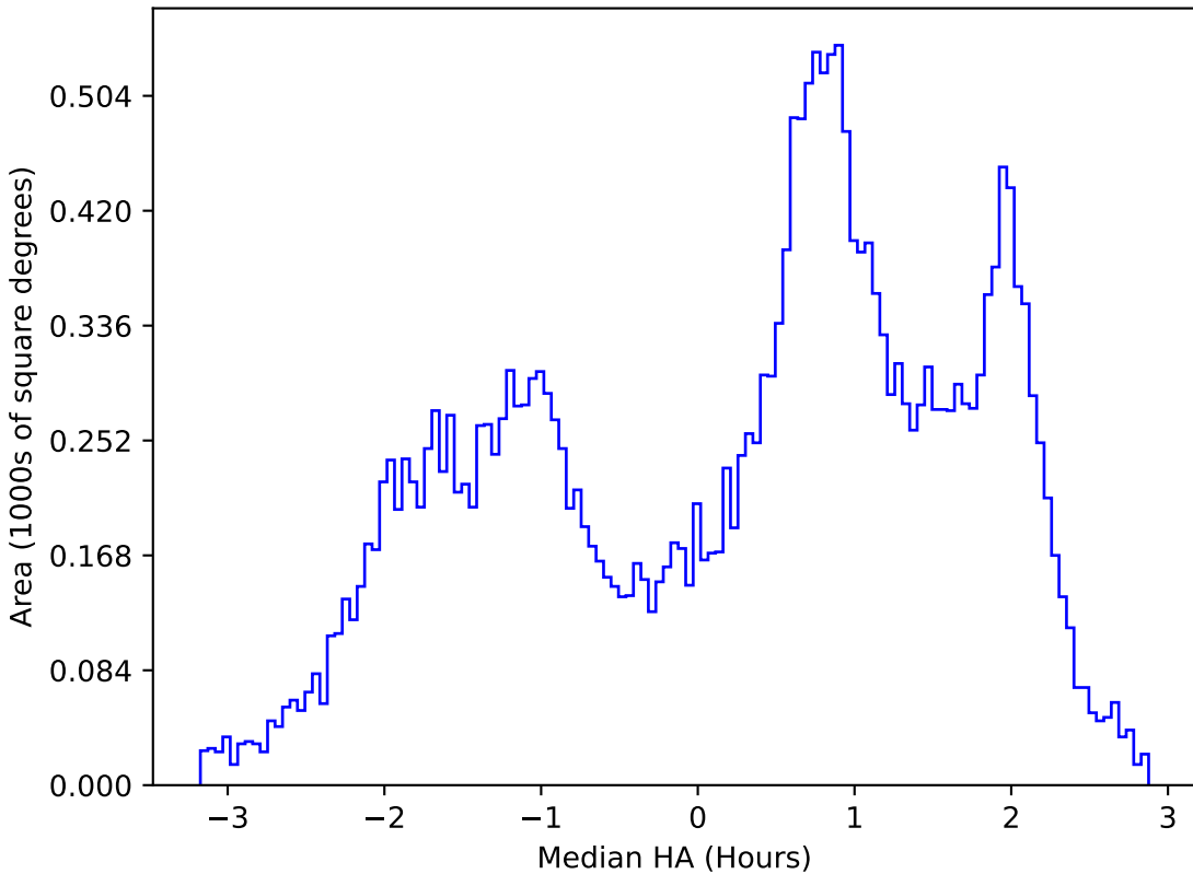
weather_cloudso35v3.4_10yrs All sky g band: Median HA
