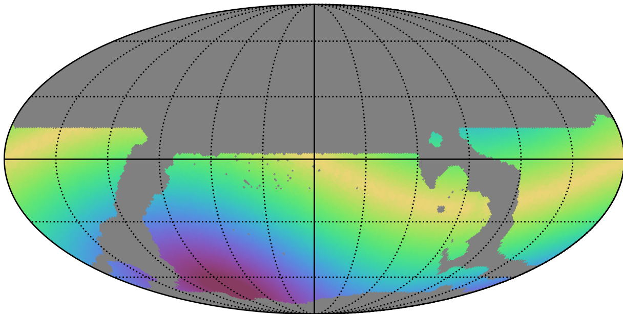
weather_cloudso35v3.4_10yrs WFD z band: Max solarElong
