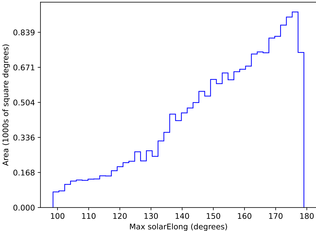
weather_cloudso35v3.4_10yrs WFD u band: Max solarElong
