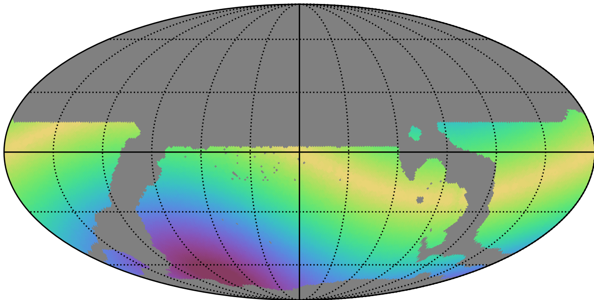
weather_cloudso35v3.4_10yrs WFD r band: Max solarElong
