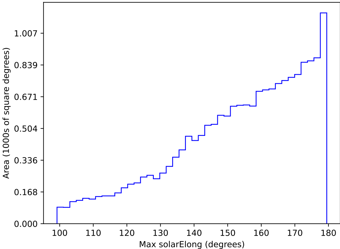
weather_cloudso35v3.4_10yrs WFD r band: Max solarElong
