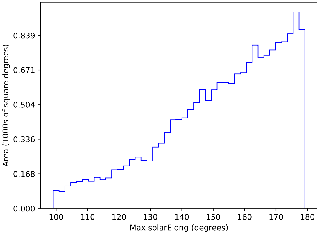
weather_cloudso35v3.4_10yrs WFD g band: Max solarElong
