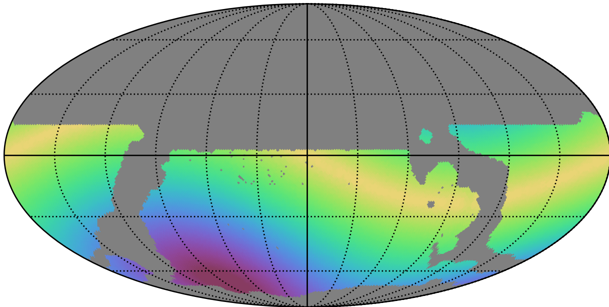
weather_cloudso35v3.4_10yrs WFD all bands: Max solarElong
