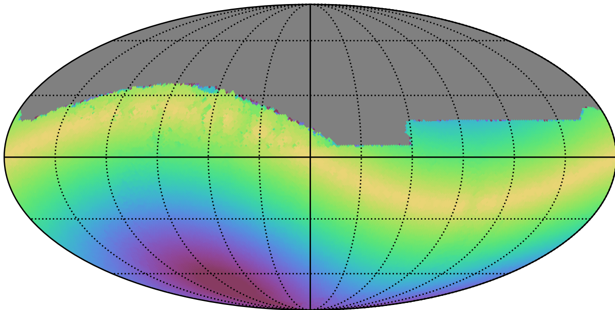
weather_cloudso35v3.4_10yrs All sky z band: Max solarElong
