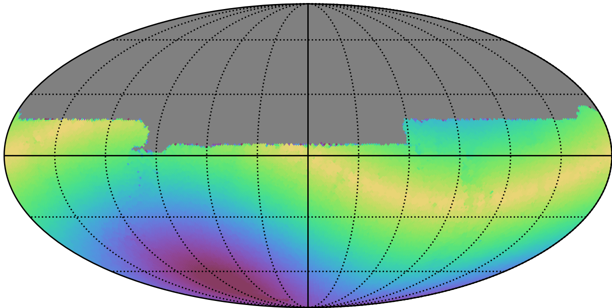
weather_cloudso35v3.4_10yrs All sky u band: Max solarElong
