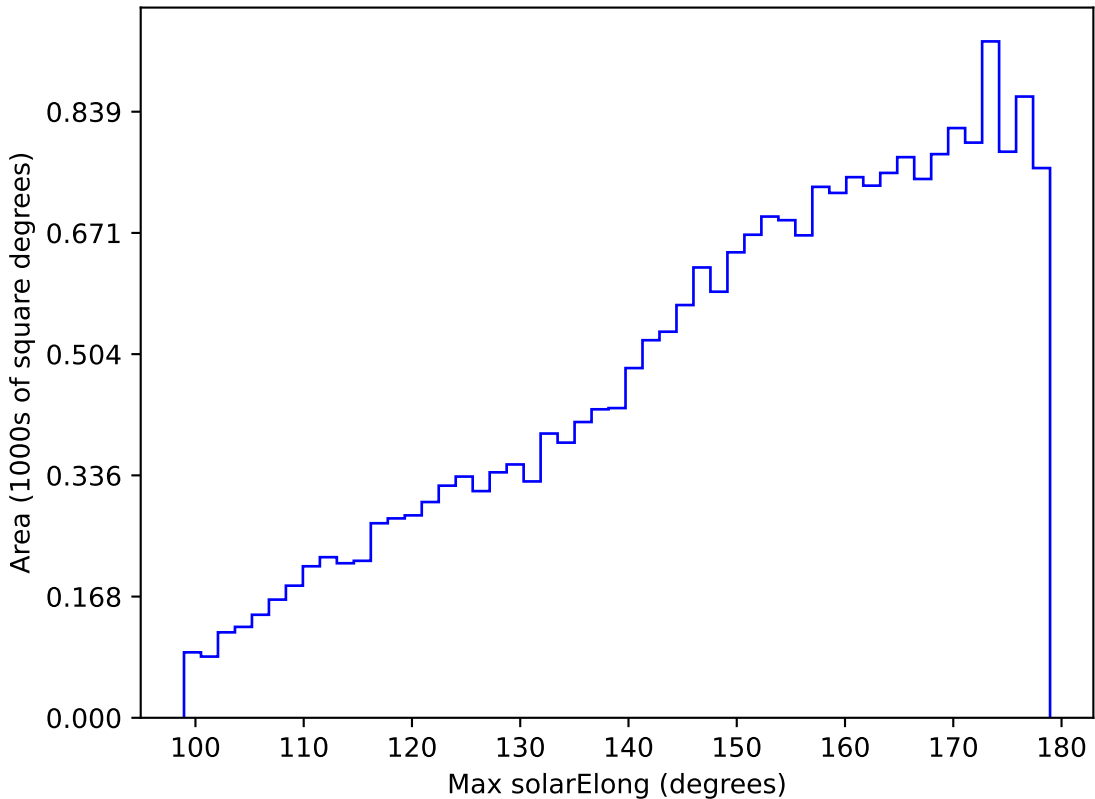
weather_cloudso35v3.4_10yrs All sky u band: Max solarElong
