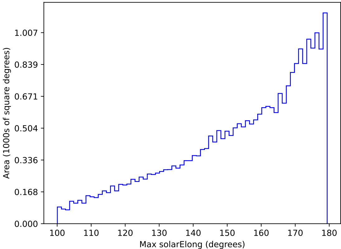
weather_cloudso35v3.4_10yrs All sky r band: Max solarElong
