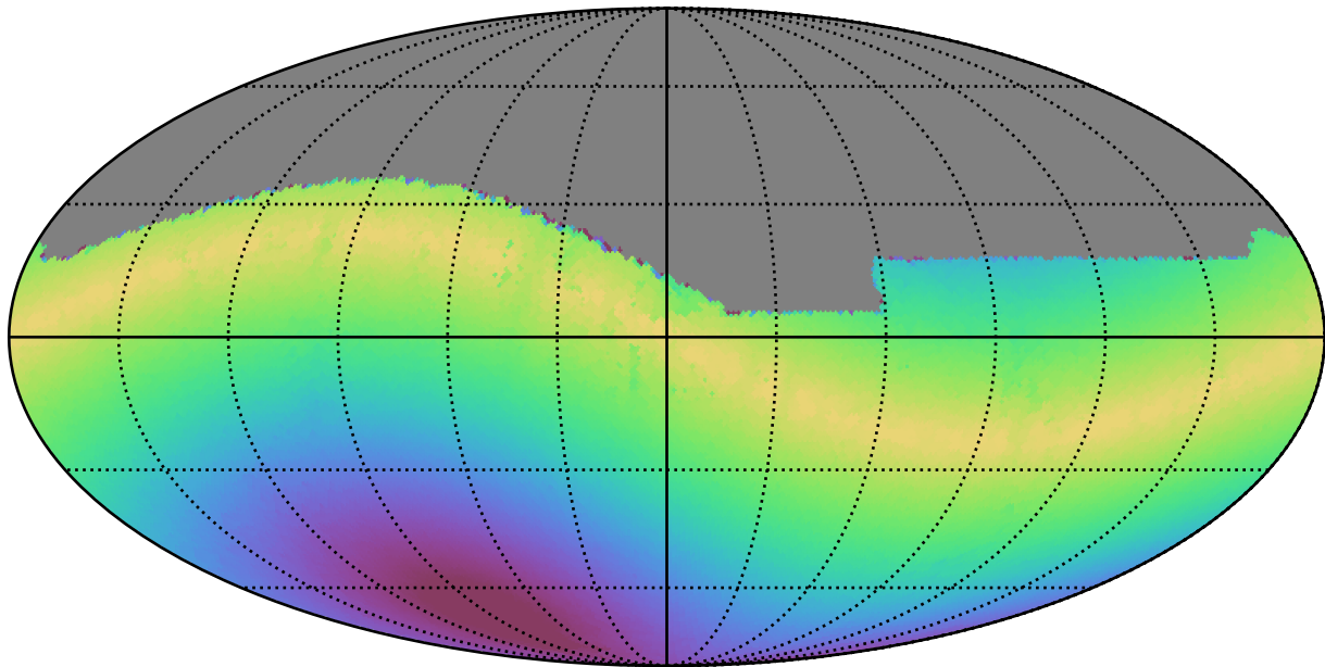
weather_cloudso35v3.4_10yrs All sky g band: Max solarElong
