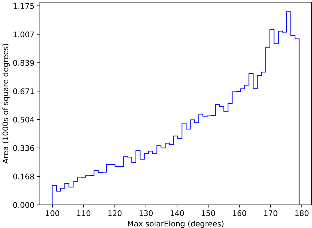
weather_cloudso35v3.4_10yrs All sky g band: Max solarElong
