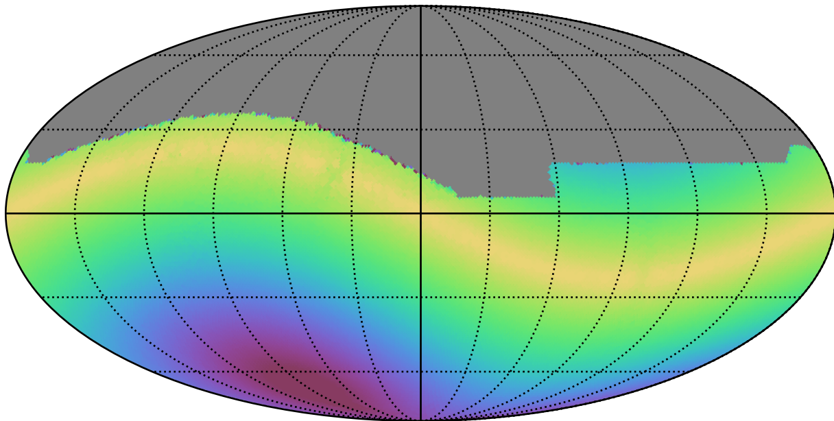
weather_cloudso35v3.4_10yrs All sky all bands: Max solarElong
