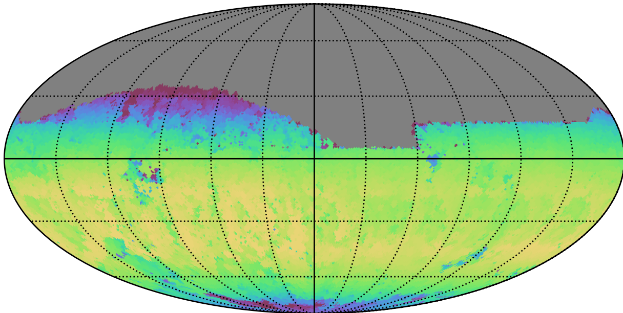
weather_cloudso35v3.4_10yrs Yr 1 z band: Max skyBrightness
