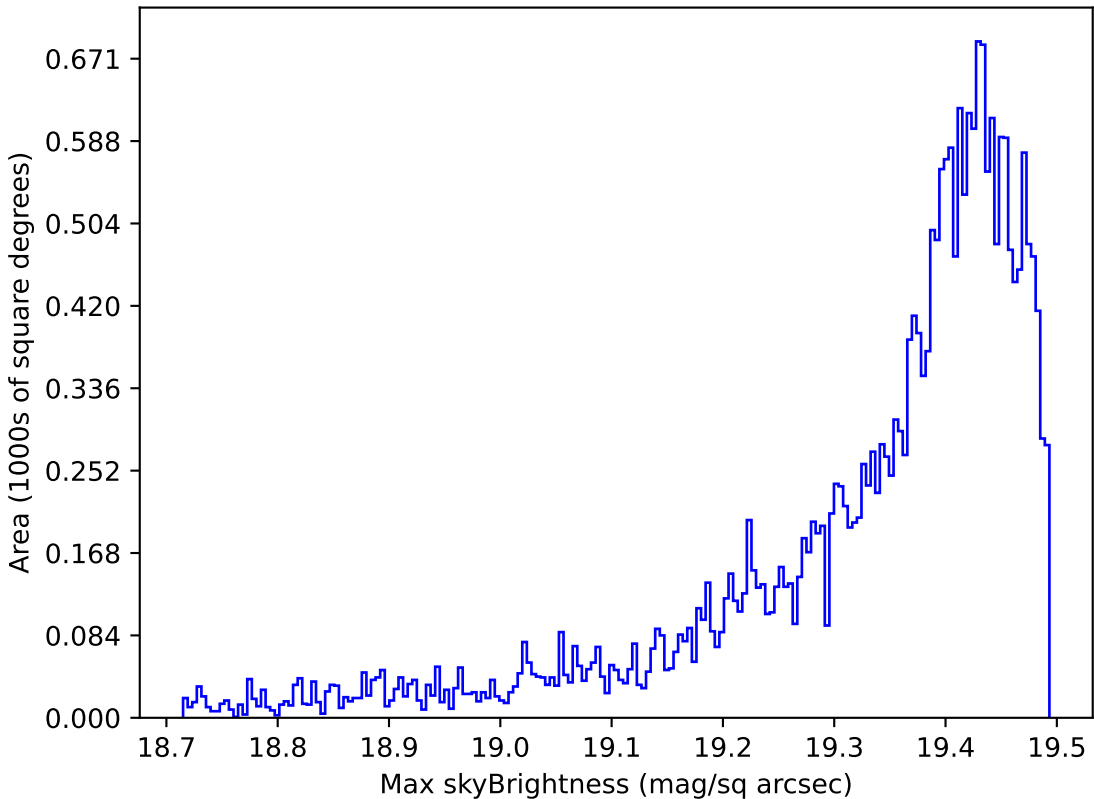
weather_cloudso35v3.4_10yrs Yr 1 z band: Max skyBrightness
