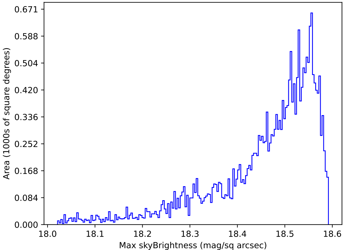
weather_cloudso35v3.4_10yrs Yr 1 y band: Max skyBrightness
