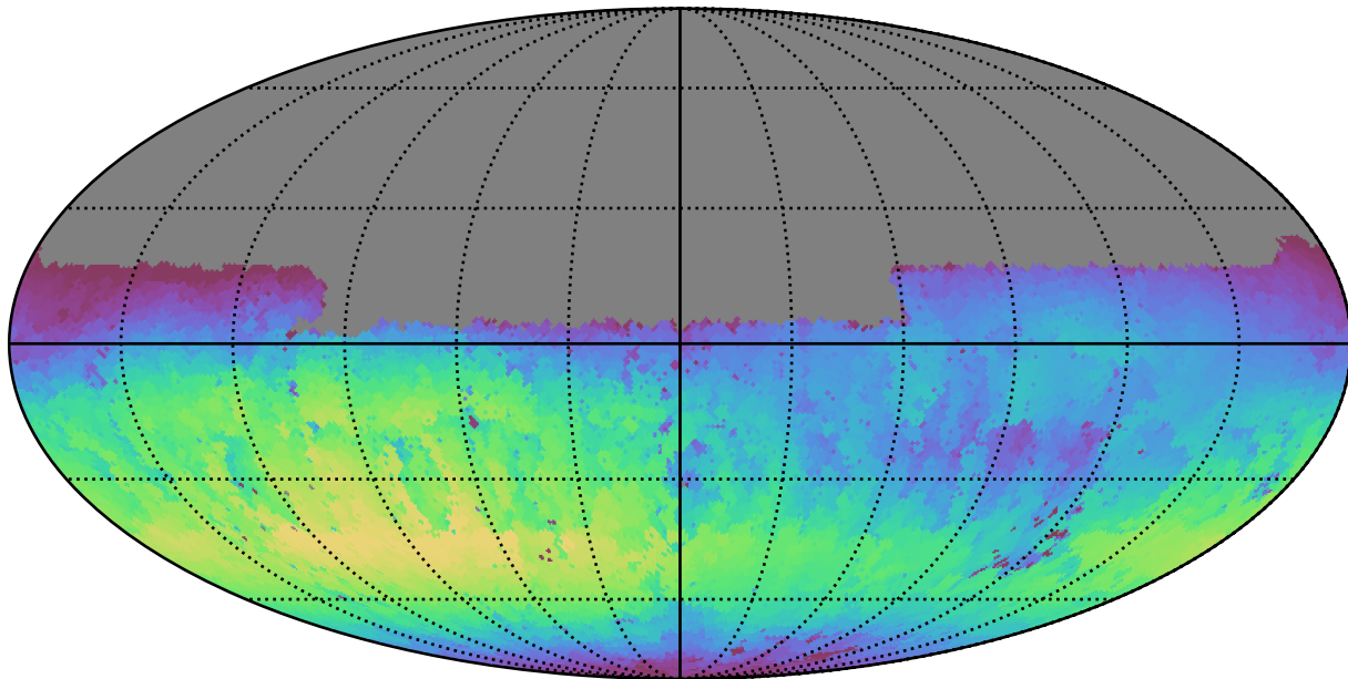
weather_cloudso35v3.4_10yrs Yr 1 u band: Max skyBrightness
