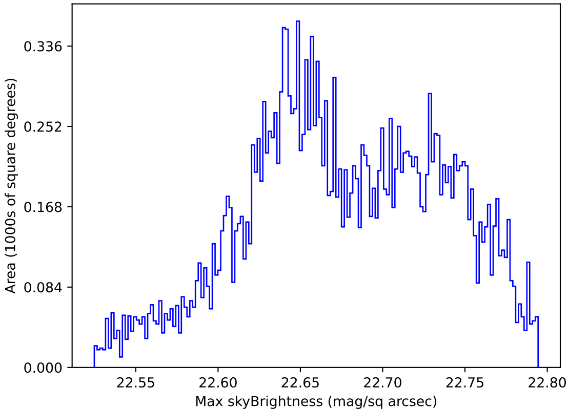
weather_cloudso35v3.4_10yrs Yr 1 u band: Max skyBrightness
