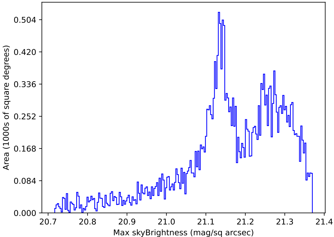
weather_cloudso35v3.4_10yrs Yr 1 r band: Max skyBrightness
