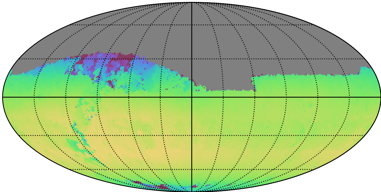
weather_cloudso35v3.4_10yrs Yr 1 i band: Max skyBrightness
