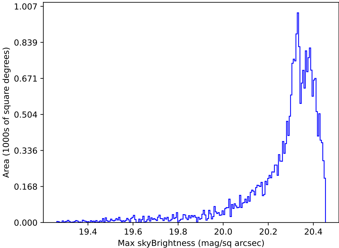
weather_cloudso35v3.4_10yrs Yr 1 i band: Max skyBrightness
