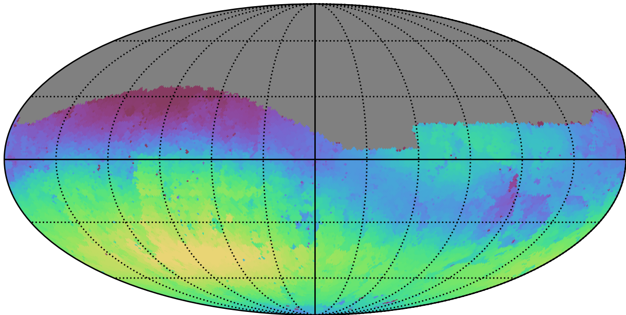
weather_cloudso35v3.4_10yrs Yr 1 g band: Max skyBrightness
