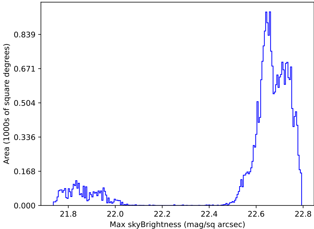
weather_cloudso35v3.4_10yrs Yr 1 all bands: Max skyBrightness
