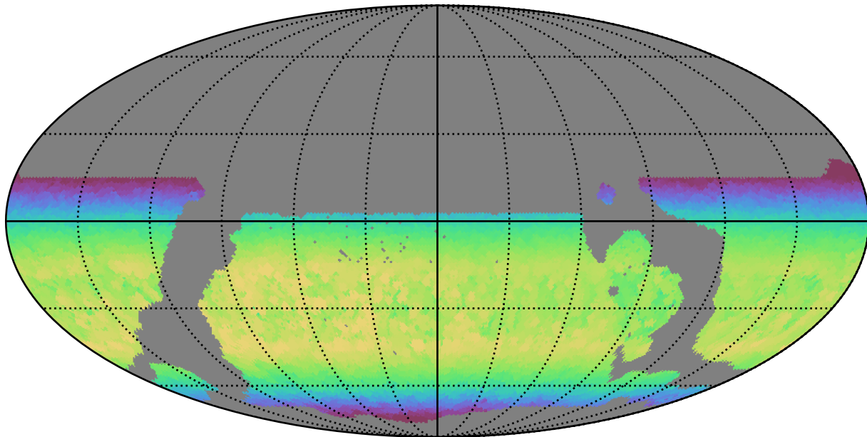
weather_cloudso35v3.4_10yrs WFD y band: Max skyBrightness
