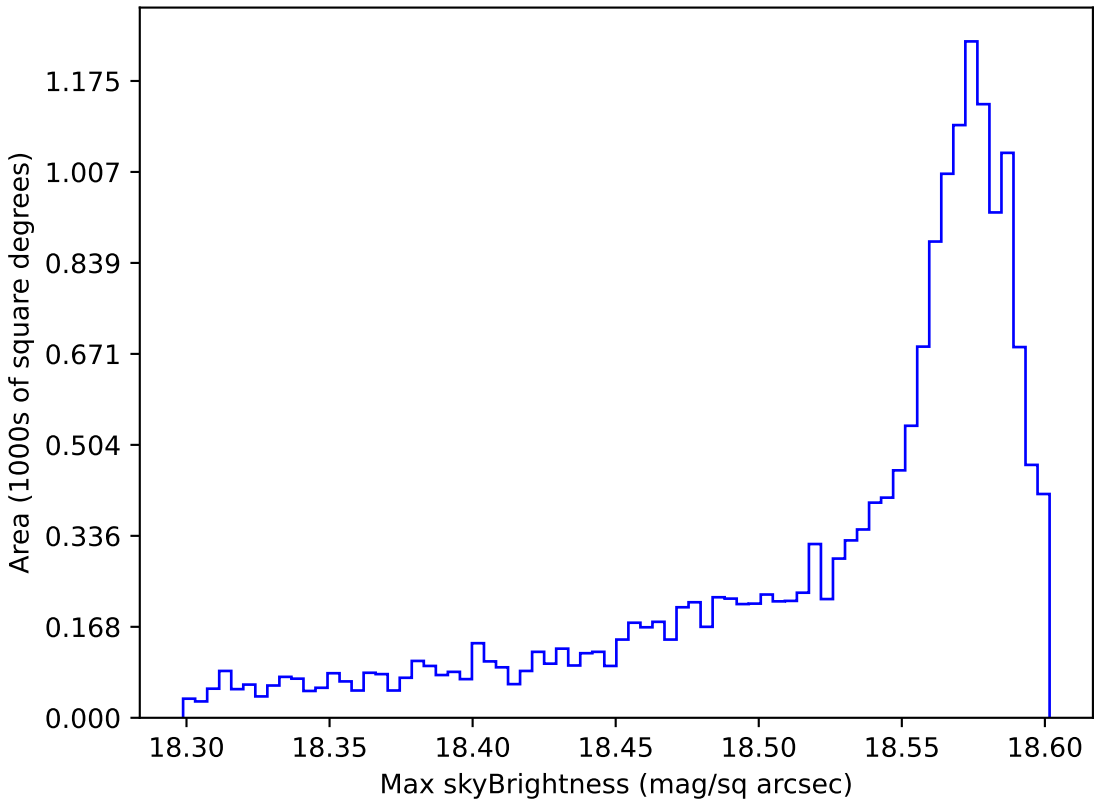
weather_cloudso35v3.4_10yrs WFD y band: Max skyBrightness
