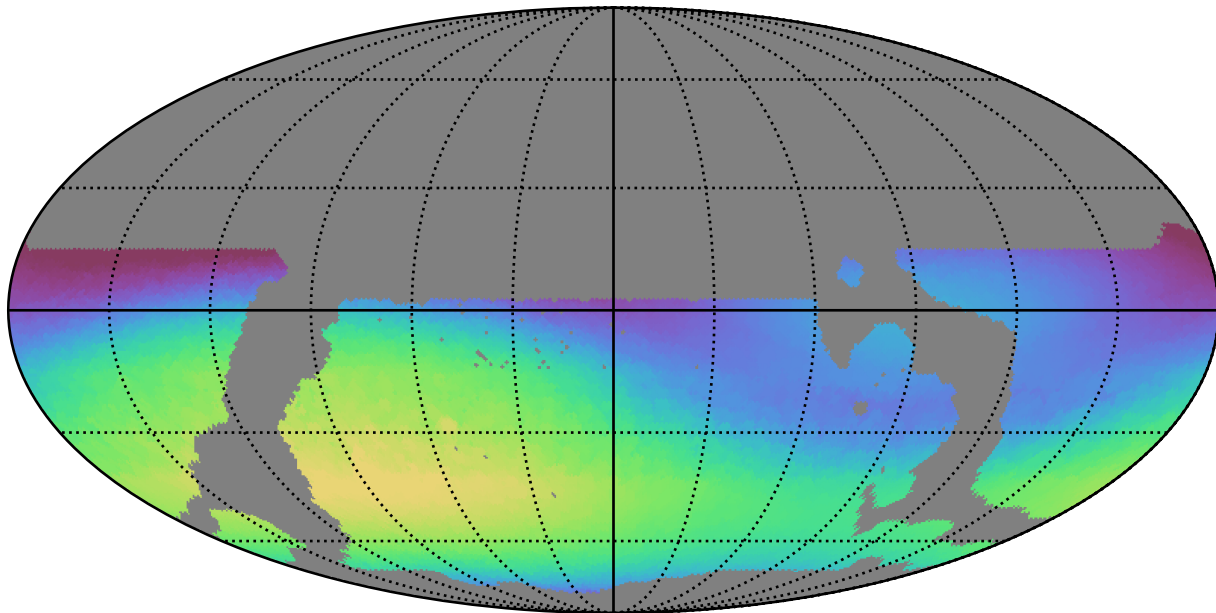
weather_cloudso35v3.4_10yrs WFD r band: Max skyBrightness
