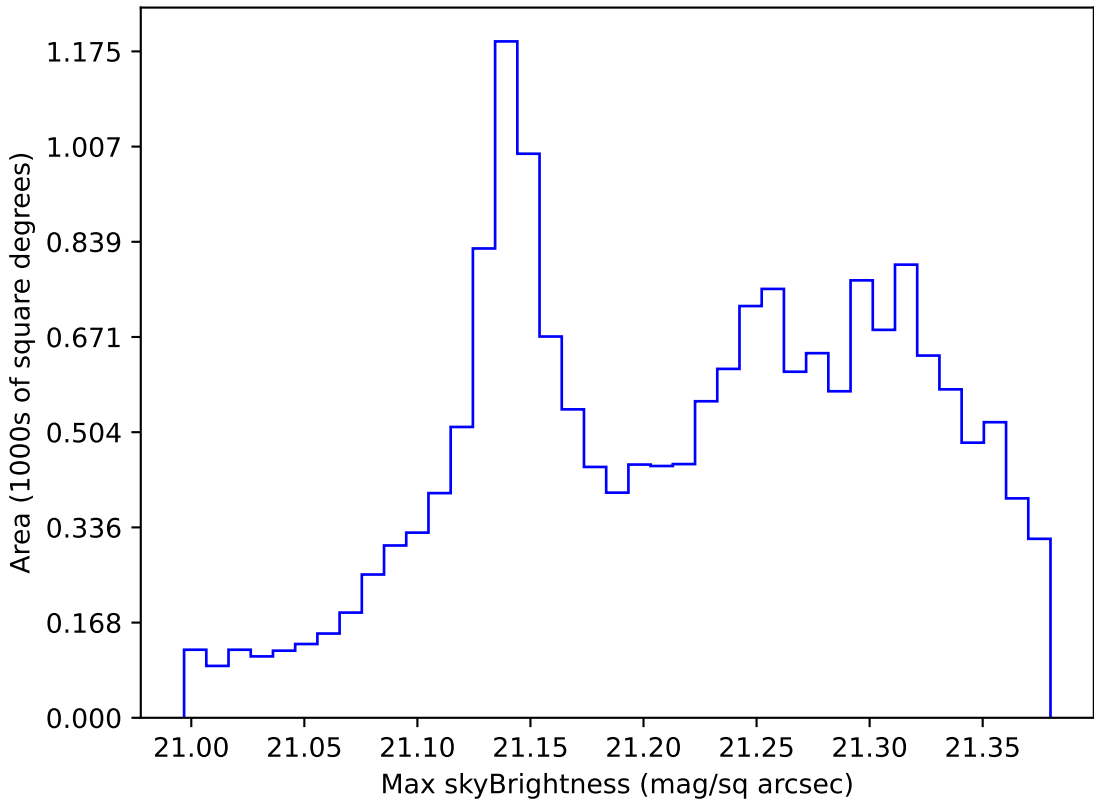
weather_cloudso35v3.4_10yrs WFD r band: Max skyBrightness
