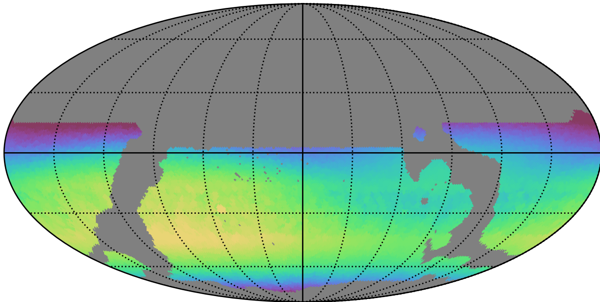
weather_cloudso35v3.4_10yrs WFD i band: Max skyBrightness
